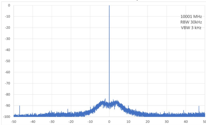
Figure 5: Non-Harmonics performance at frequencies non-fractional to the reference, 10 001 MHz
