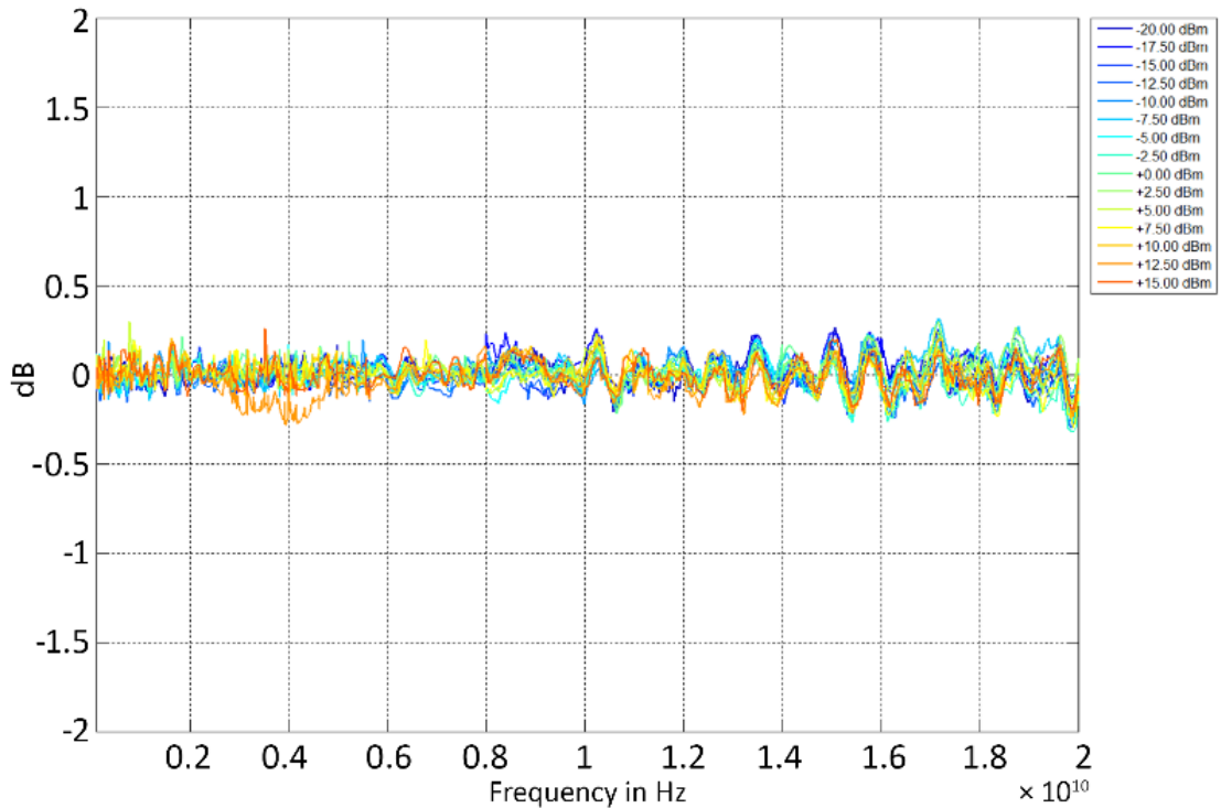
Figure 11: Level accuracy over frequency (APLC20)
