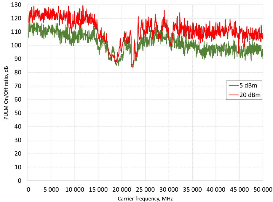
Figure 16: Polarity Pulse On / Off ratio at +10dBm output power and 20 ns pulse
