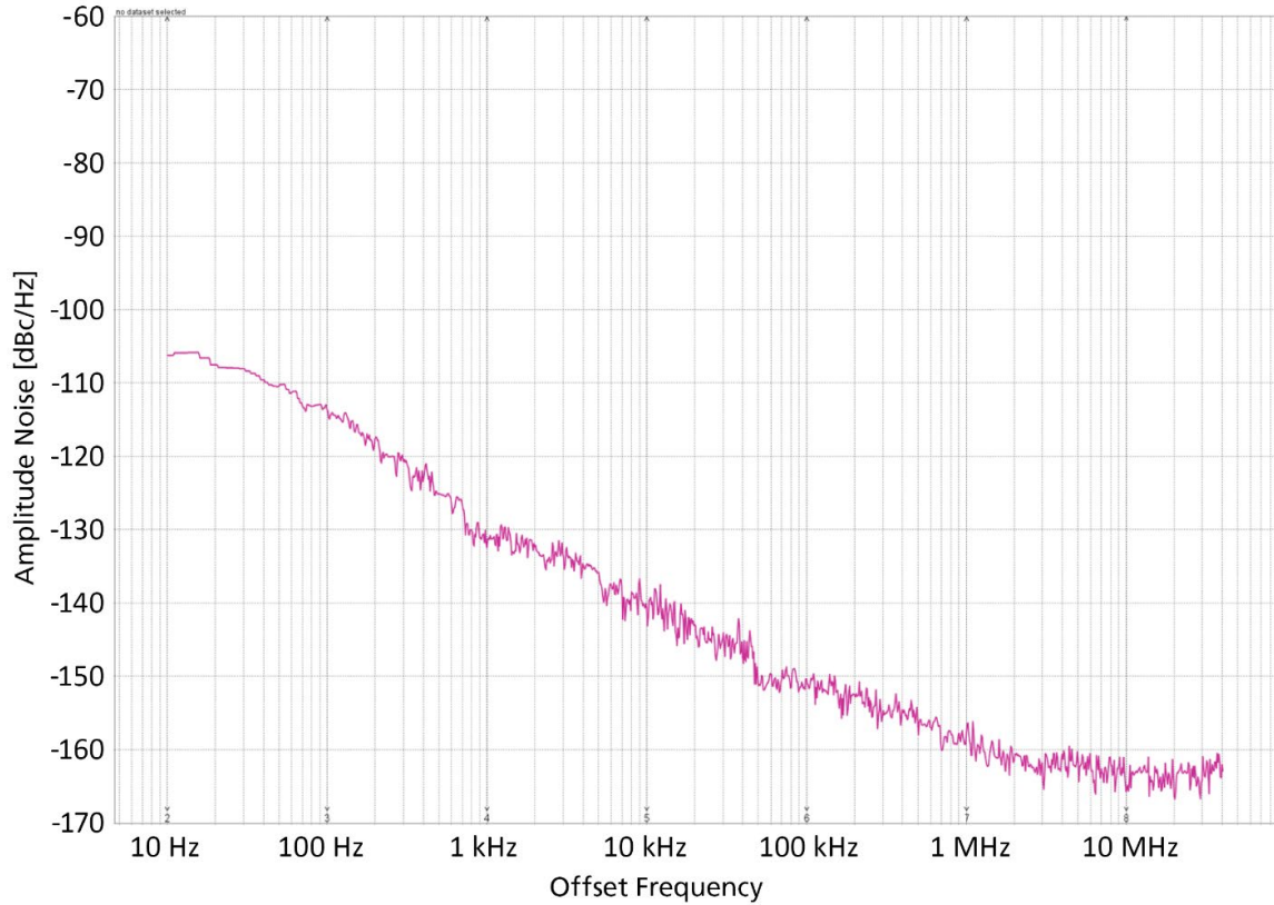
Figure 2: Amplitude Noise at 10 GHz, power +10 dBm
