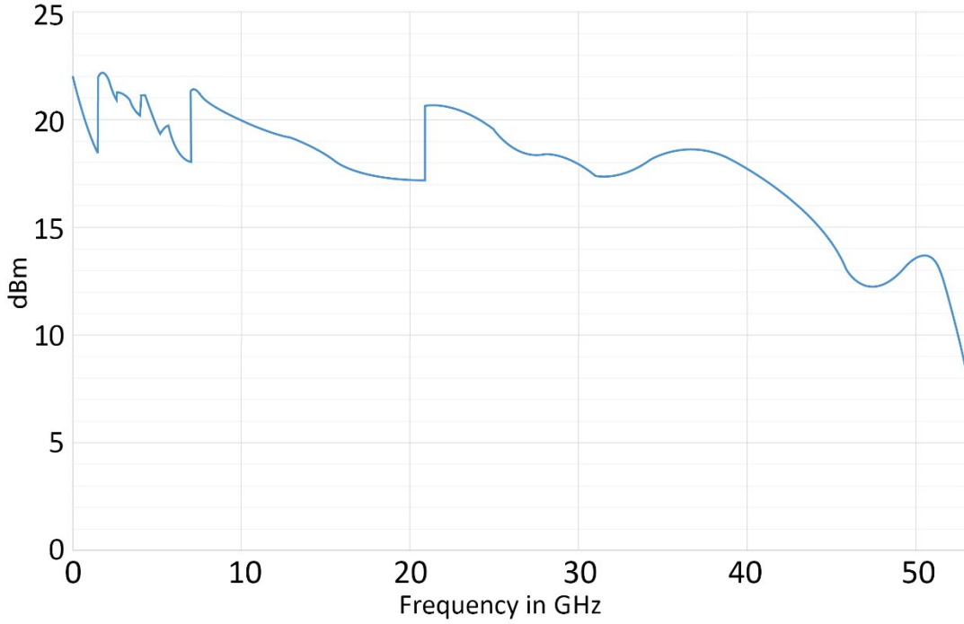
Figure 10: Maxpower 100 MHz to 54 GHz (option PE2)
