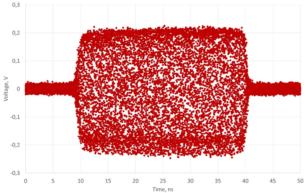
Figure 18: 50 GHz pulse modulation 30 ns
