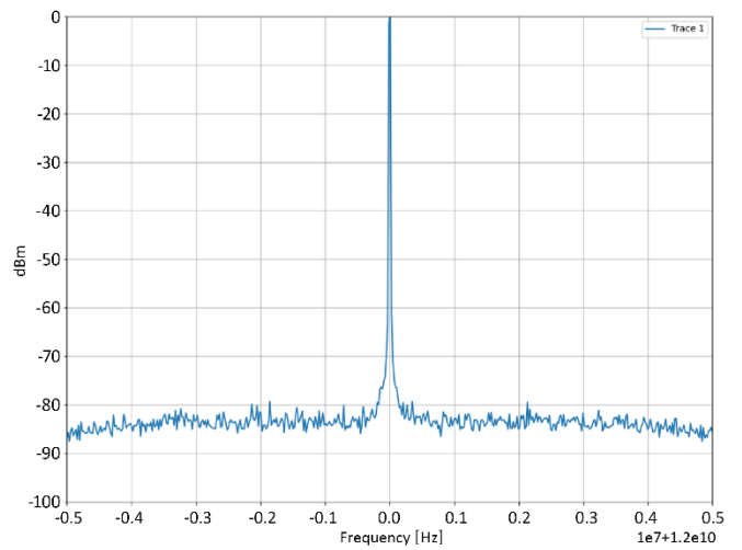
Figure 4: Non-Harmonic Spurs (12 GHz)
