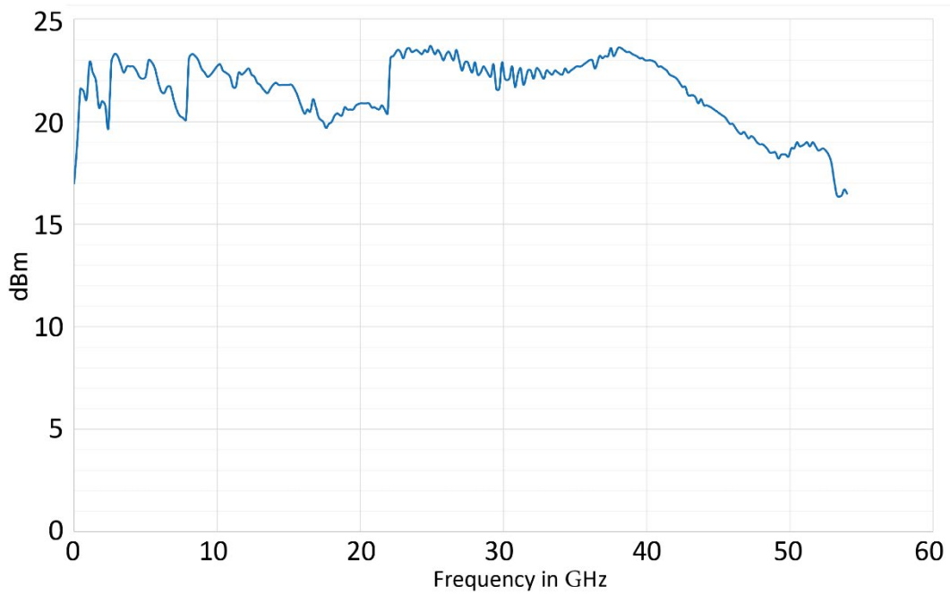
Figure 9: Maxpower 100 MHz to 54 GHz (standard)
