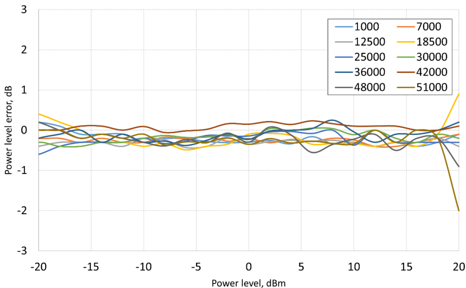
Figure 13: Power Linearity at different frequencies
