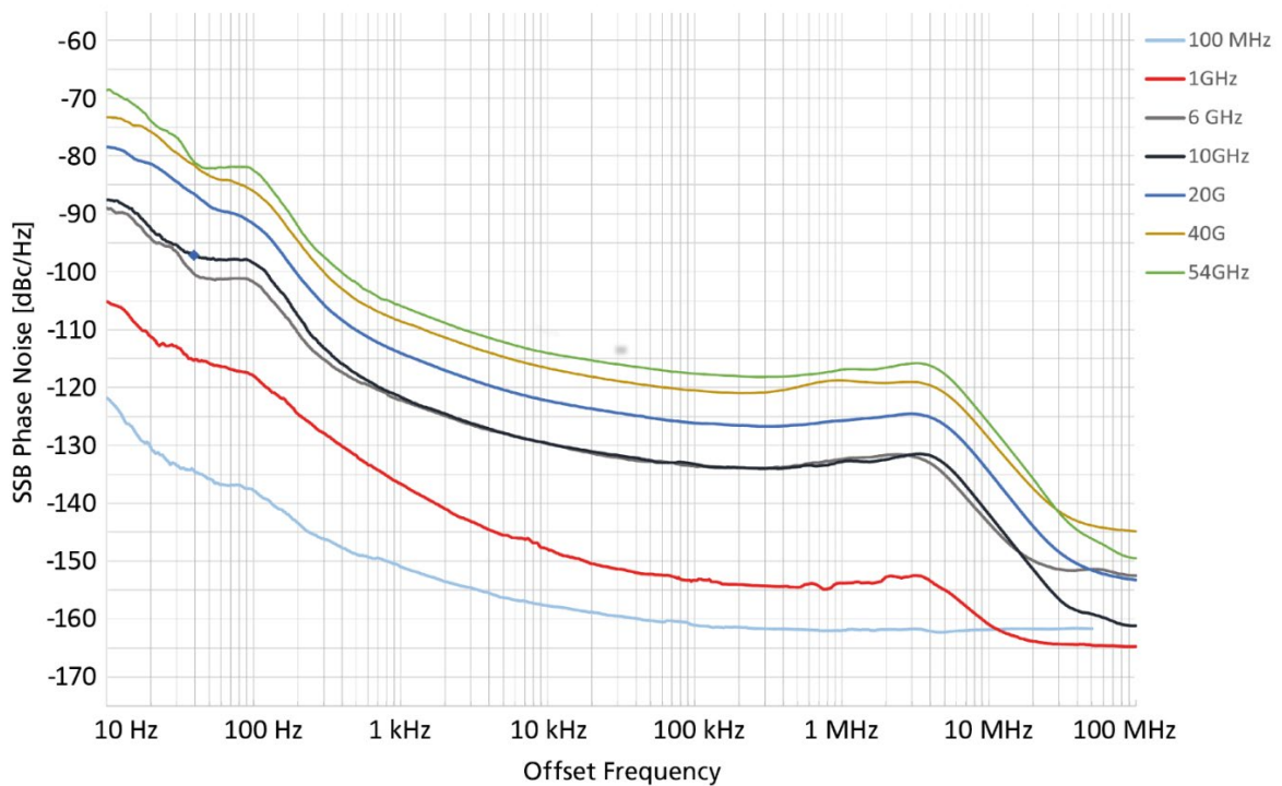
Figure 1: Phase Noise at different frequencies, power +10 dBm, Option LN
