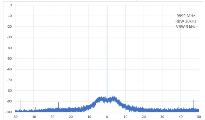
Figure 6: Non-Harmonics performance at frequencies non-fractional to the reference, 9999 MHz
