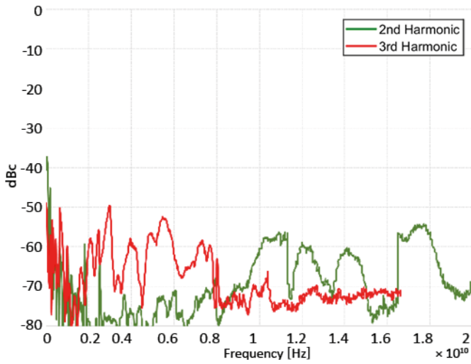
Figure 3: Harmonics at +10 dBm
