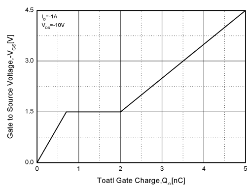
Figure6. Gate Charge
