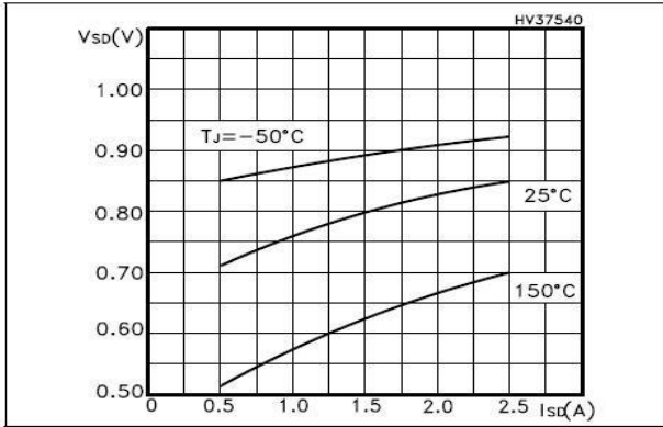
Figure 16. Source-drain diode forward characteristics
