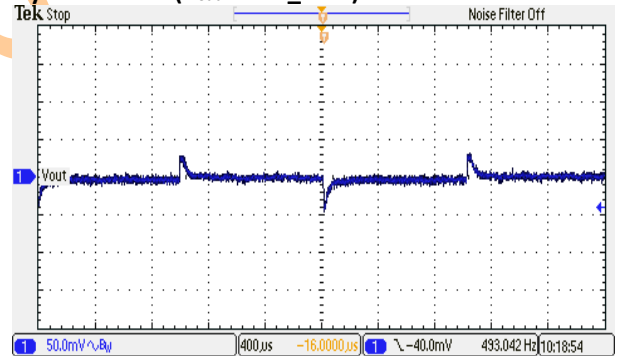
Dynamic Load ( I_{Load}=0.2A\_1.2A )
