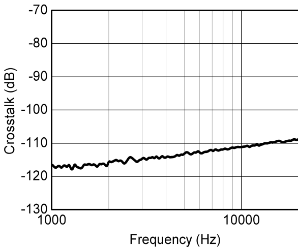
Crosstalk
