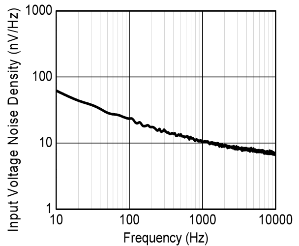
Noise Density
