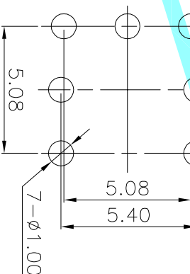
PCBLayout(Pattern Side)
