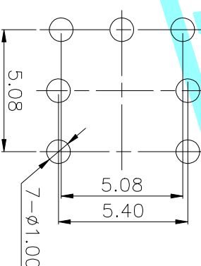
PCBLayout(Pattern Side)
