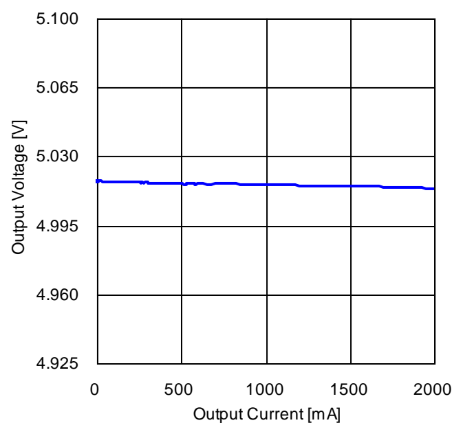
Figure 87. Load Regulation (V IN = 12 V)
