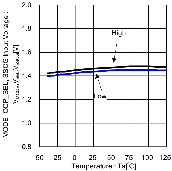
Figure 17. MODE, OCP_SEL, SSCG Input Voltage vs Temperature
