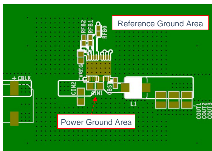
Figure 90. Recommended Board Layout Example (for BD9P2x5EFV-C)
