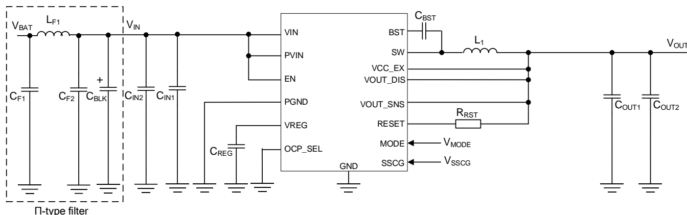
Figure 75. Reference Circuit 3
