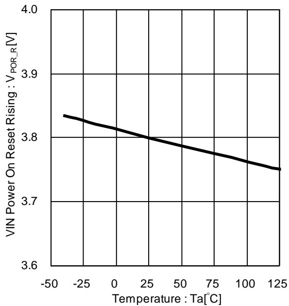
Figure 13. VIN Power On Reset Rising vs Temperature
