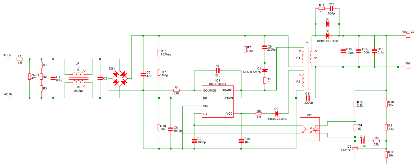
Figure 25. BM2P10B1J-EVK-001 Schematics
