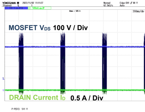
Figure 15. V_{DS} , I_D V_{IN} = 264 \text{ Vac} , V_{OUT} Shorted
