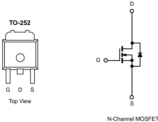
N-Channel MOSFET
