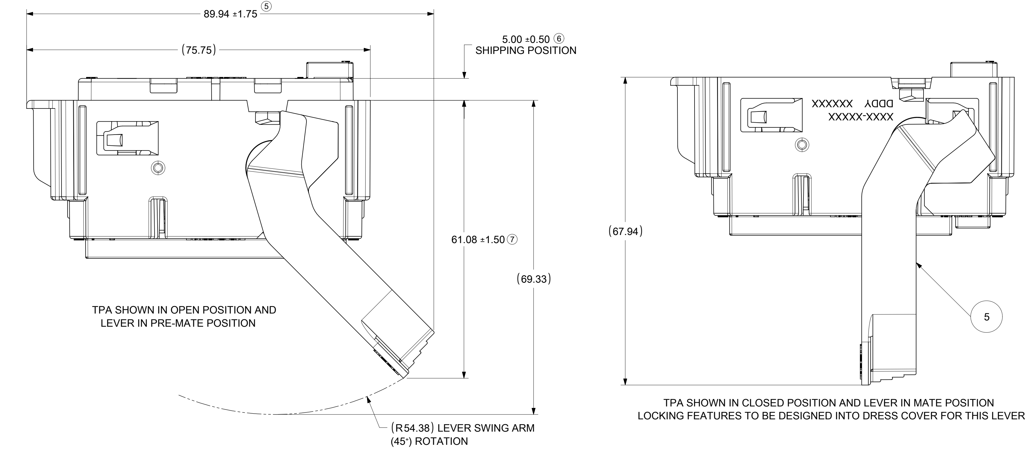
VIEW SHOWN WITHOUT MOLDED IN CAVITY PLUGS
