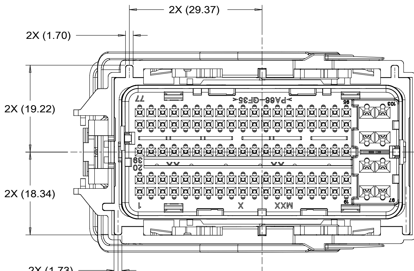
34993-8XXX (END LATCH LEVER) 34993-9XXX (TOP LATCH LEVER) KEY OPTION 5
