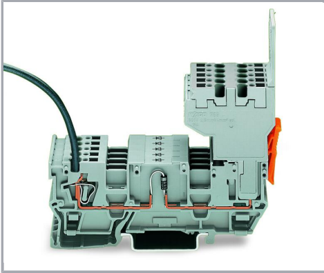
2-conductor female plug Diode carrier terminal blocks can be commoned via 280 and 780 Series Jumpers and tested using a test plug adapter (280-4..).
