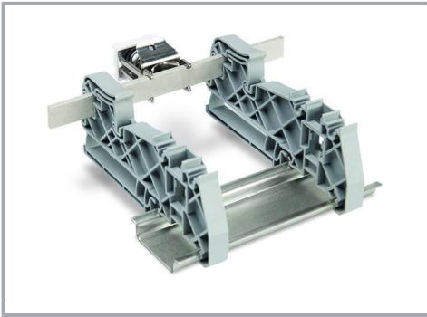
Vertical mounting position of the busbar
