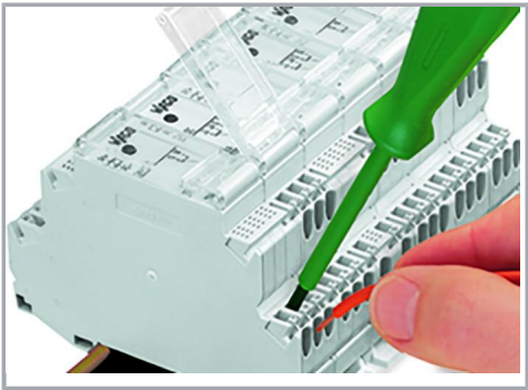
Inserting a conductor.
