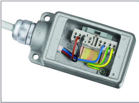
Wiring example in an Ex junction box
