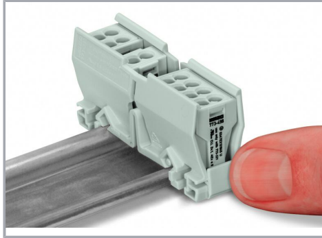
Use the cover as an end plate.
