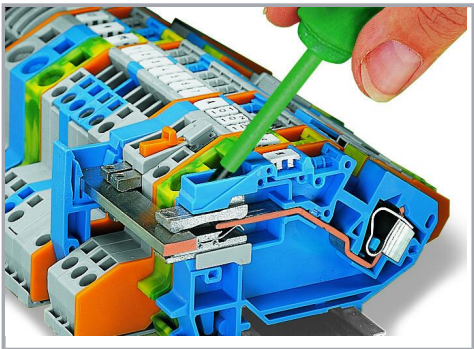
Operating a screwless N-disconnect slide link.
