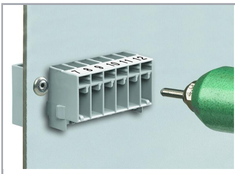
Mounting with 3 mm Ø blind rivets
