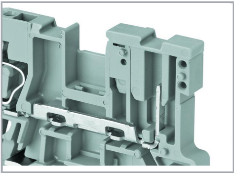
Pin cover (769-438) with Mini-WSB marker slot
