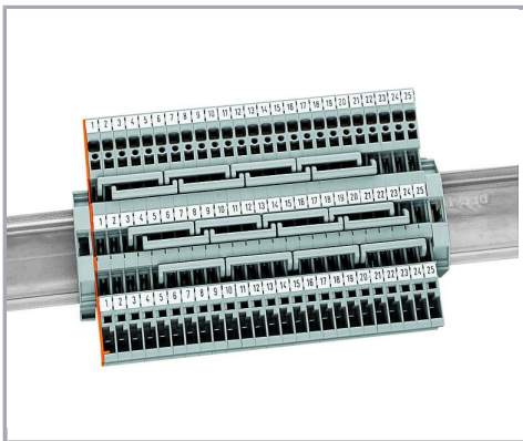
1-conductor/1-pin carrier terminal blocks with three jumper positions The three jumper positions allow up to six commoning options for staggered jumpers.
