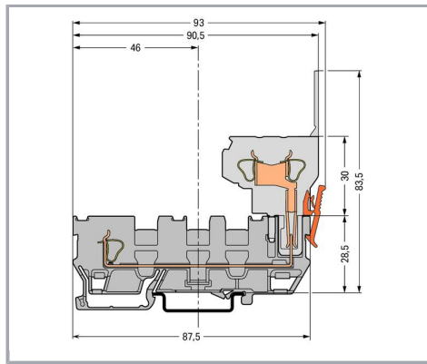
Carrier terminal block For dimensions, see carrier terminal block (769-171).
