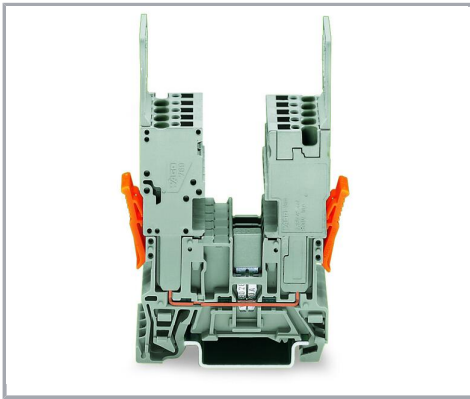
1-conductor female plugs Carrier terminal blocks can be commoned via 280 and 780 Series Jumpers and tested using a test plug adapter (280-4..).
