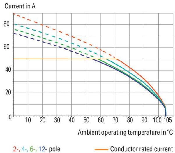
Current-Carrying Capacity Curve Conductor – Solder Pin Pin spacing: 7.5 mm / Conductor cross-section: 10 mm 2 "f-st" Based on: EN 60512-5-2 / Reduction factor: 1
