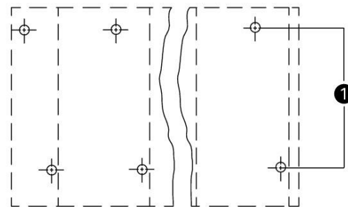
(1) Solder pins staggered by half the pin spacing
