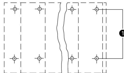
(1) Solder pins in line
