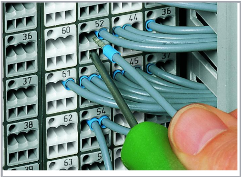
CAGE CLAMP® connection Terminating ferruled conductors via operating tool.
