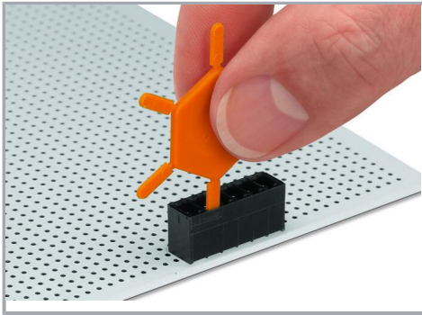
Coding a male header by inserting a coding pin. (MCS MINI SL)
