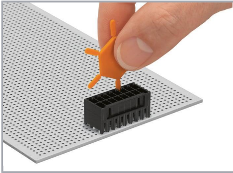
Coding a male header by inserting a coding pin. (MCS MINI HD)
