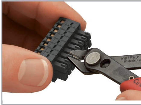
Coding a female connector by removing coding finger(s). (MCS MINI HD)
