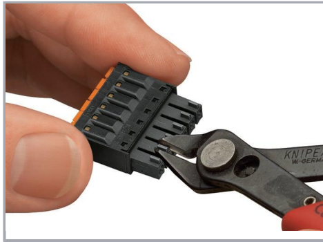
Coding a female connector by removing coding finger(s). (MCS MINI SL)
