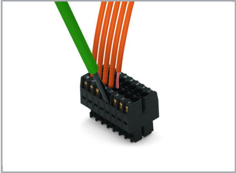
Inserting a conductor via (2.5 x 0.4) mm screwdriver.
