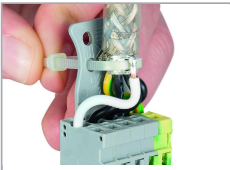
Secure both shield cable and shield termination to the strain relief plate using cable ties.
