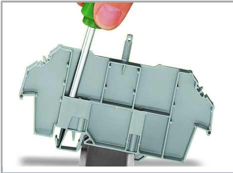
Removing a cover carrier from the DIN-rail.
