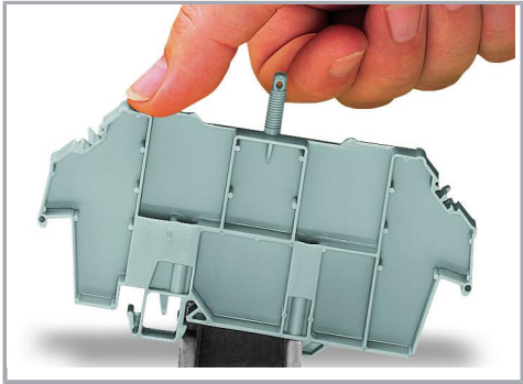
Snapping a cover carrier onto the DIN-rail.
