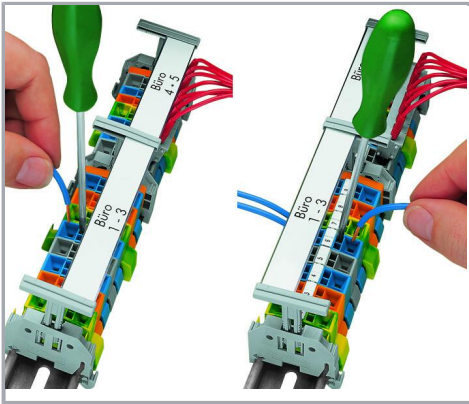
Laterally movable marking system
