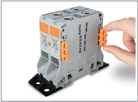
Optionally, insert block-to-block connector (285-168) into housing slot.
