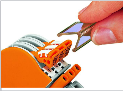
Snapping transparent locking cover onto 1–8 disconnect links:
