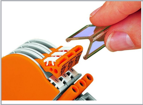
Snapping transparent locking cover onto 1–8 disconnect links: a) Mechanically lock several links for multi-pole switching applications b) Protect markers
