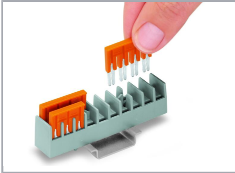
Collective jumper carrier Inserting a jumper.
