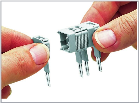
Snapping test plug and spacer modules together to assemble a multipole test plug module (max. 10 poles).
