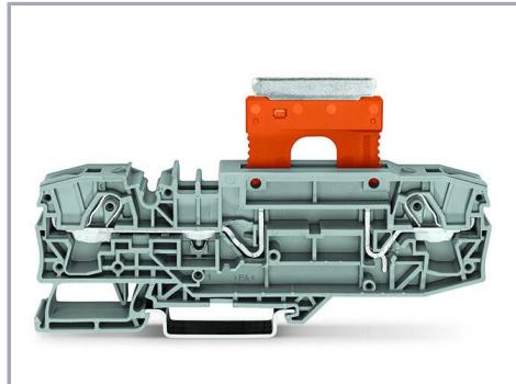
Carrier terminal block with disconnect plug (2006-8401) in parked position
