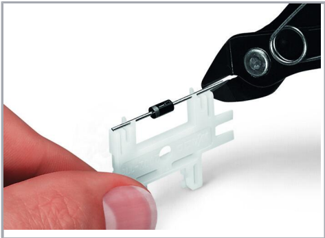
Cutting component to the proper length.
