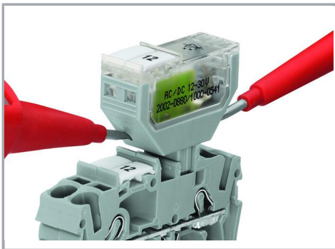
Testing Can also be performed using 2-pole test plugs.
