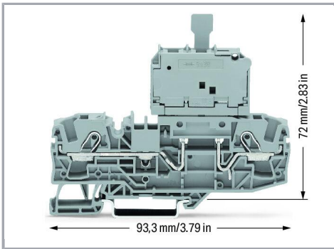
Fuse plug dimensions
