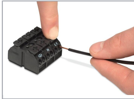
Inserting a conductor via push-button.
