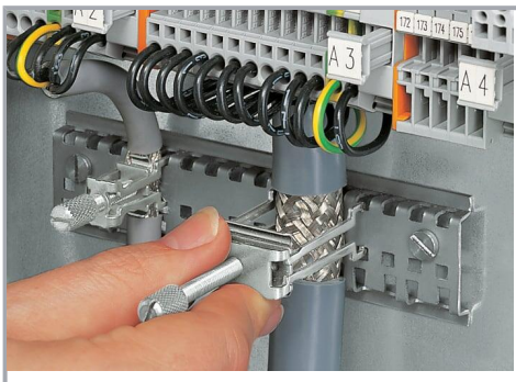
Securing an additional shield clamping saddle.
