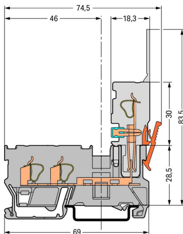
Carrier terminal block
