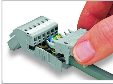
Snapping on a strain relief housing.
