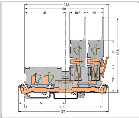
Securing a female plug via locking lever on the terminal block side.
