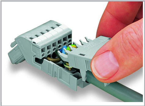
Snapping on a strain relief housing.
