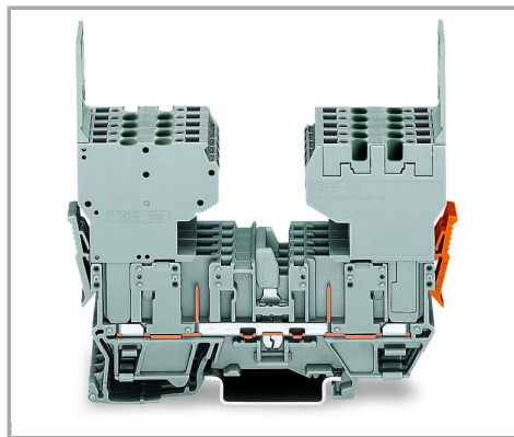
2 x 2-conductor female plugs Carrier terminal blocks can be commoned via 280 and 780 Series Jumpers and tested using a test plug adapter (280-4..).
