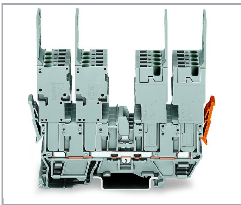
4 x 1-conductor female plugs Carrier terminal blocks can be commoned via 280 and 780 Series Jumpers and tested using a test plug adapter (280-4..).
