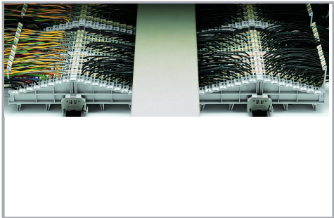
Example of matrix patching assembly Left: Main cables fed through locking clips on the field side Right: Control cables fed between locking clips Center: Wiring of both patching sides
