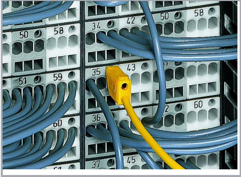
Testing with a 2.3 mm Ø test plug (210-137).
