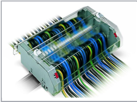
Application example: Cover (type 1) without safety warning
