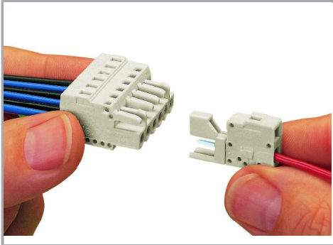
Test plug adapter with CAGE CLAMP® connection
