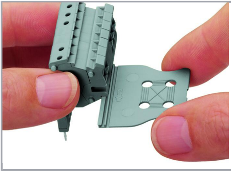
Snapping on a strain relief plate.
